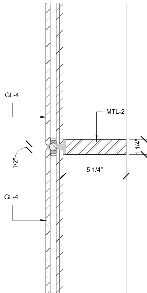
4 LOBBY HORIZONTAL MULLION DETAIL - SECTION 3" = 1'-0"
